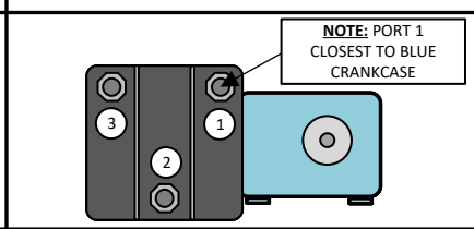
DETAIL VIEW 1: Side View Of Pearson Pump
