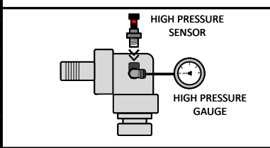
DETAIL VIEW 2: High Pressure Sensor & Gauge
