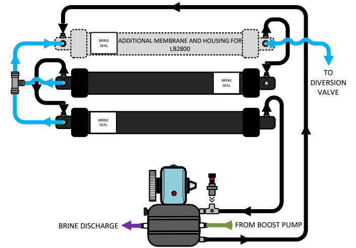
DETAIL VIEW 4: LB2800 Membrane Array Plumbing
