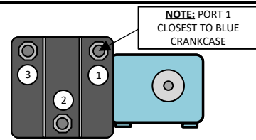
DETAIL VIEW 1: Side View Of Pearson Pump
